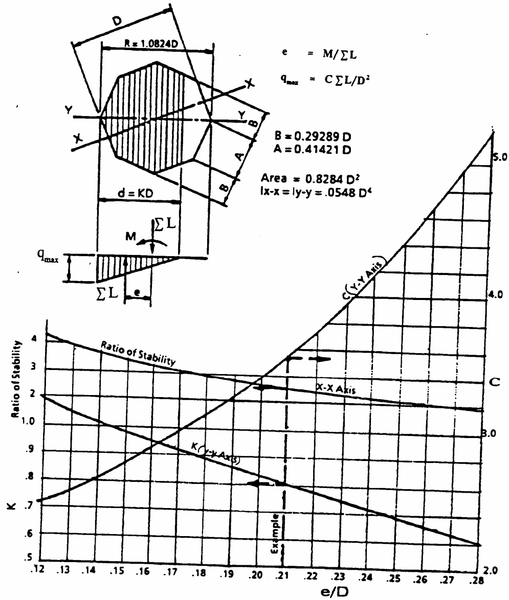
Soil Bearing Pressure co-efficient for octagonal footing (Reference from text book)
